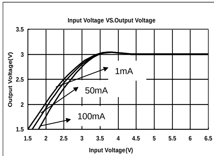
ME6211C30M5G
