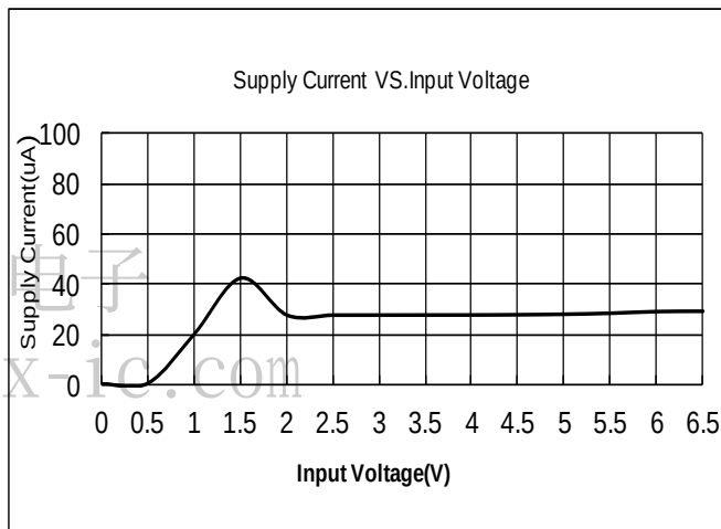
ME6211C18M5G
