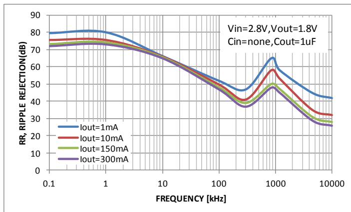
ME6211C18M5G
