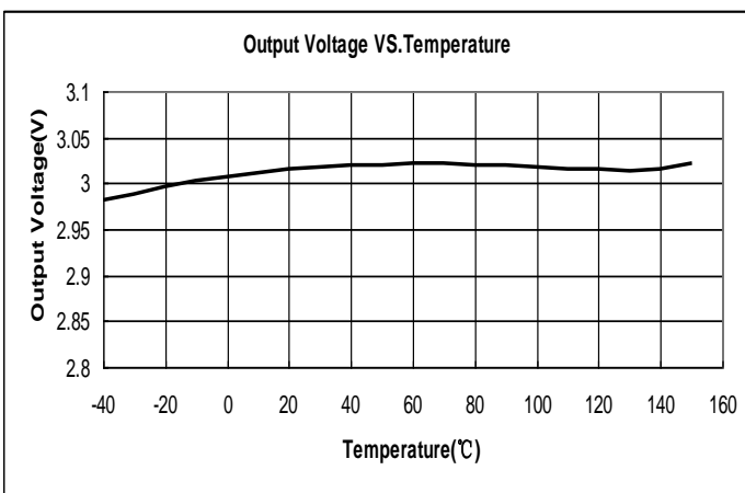
(5) Output Voltage VS. Temperature
