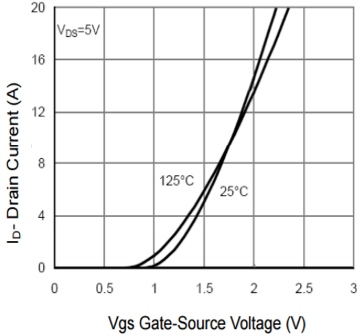
Figure 7 Transfer Characteristics
