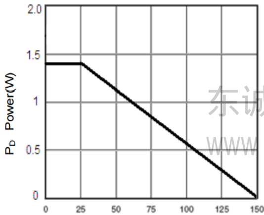
Figure 3 Power Dissipation
