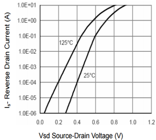
Figure 12 Source- Drain Diode Forward
